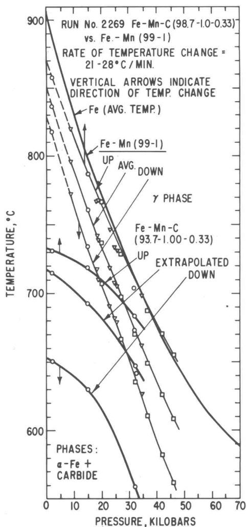
Fig. 13 P-T plots for Fe-Mn-C eutectoid reaction. Extrapolated temperatures and temperature hysteresis
